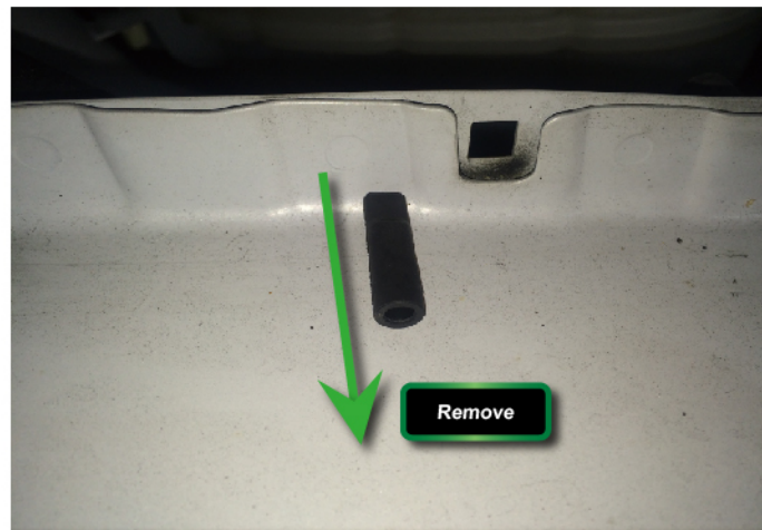
▶4.Remove the plug of preserved vacuum port
